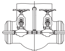
With equalizing pipe and bypass valves
