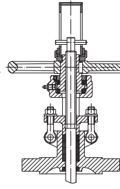
Position indicator
